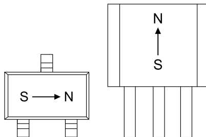
Figure 2. Sensing direction
