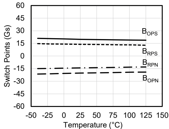
Figure 15. Switch points versus temperature ( V_{CC} = 3\text{ V} )
