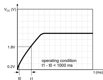
Figure 19. Power up timing
