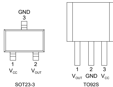
Figure 4. Pin configuration
