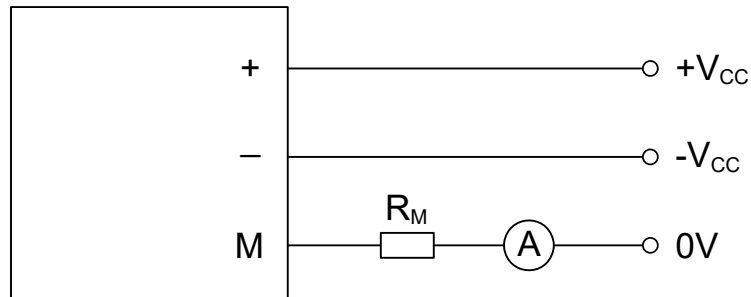
Figure 1. Electrical Connection
