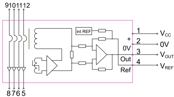
Figure 18. TMR7304-D Electrical Connection
