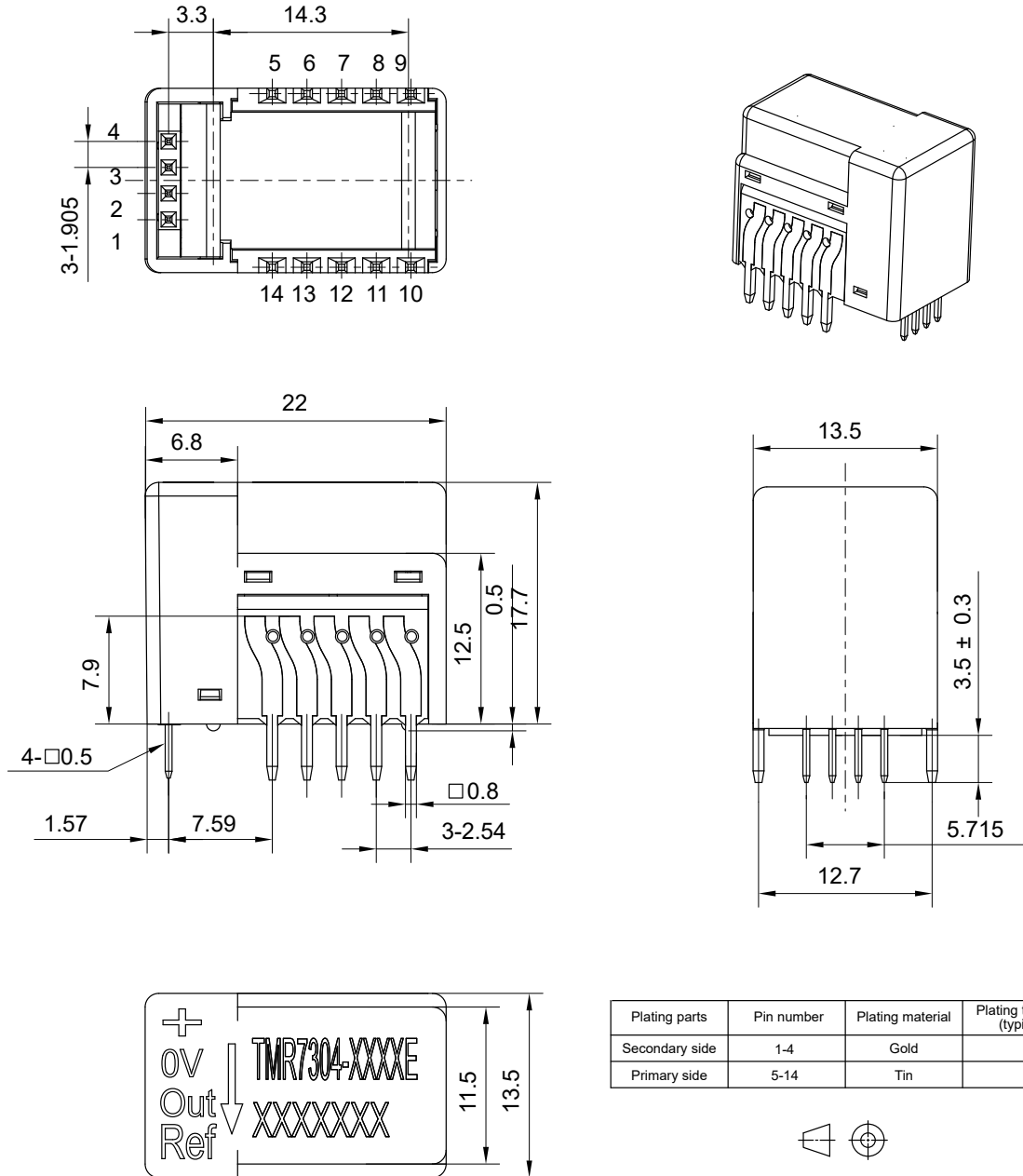
Figure 23. Dimension for TMR7304-E (unit: mm, tolerances for unmarked scales \pm 1 mm)
