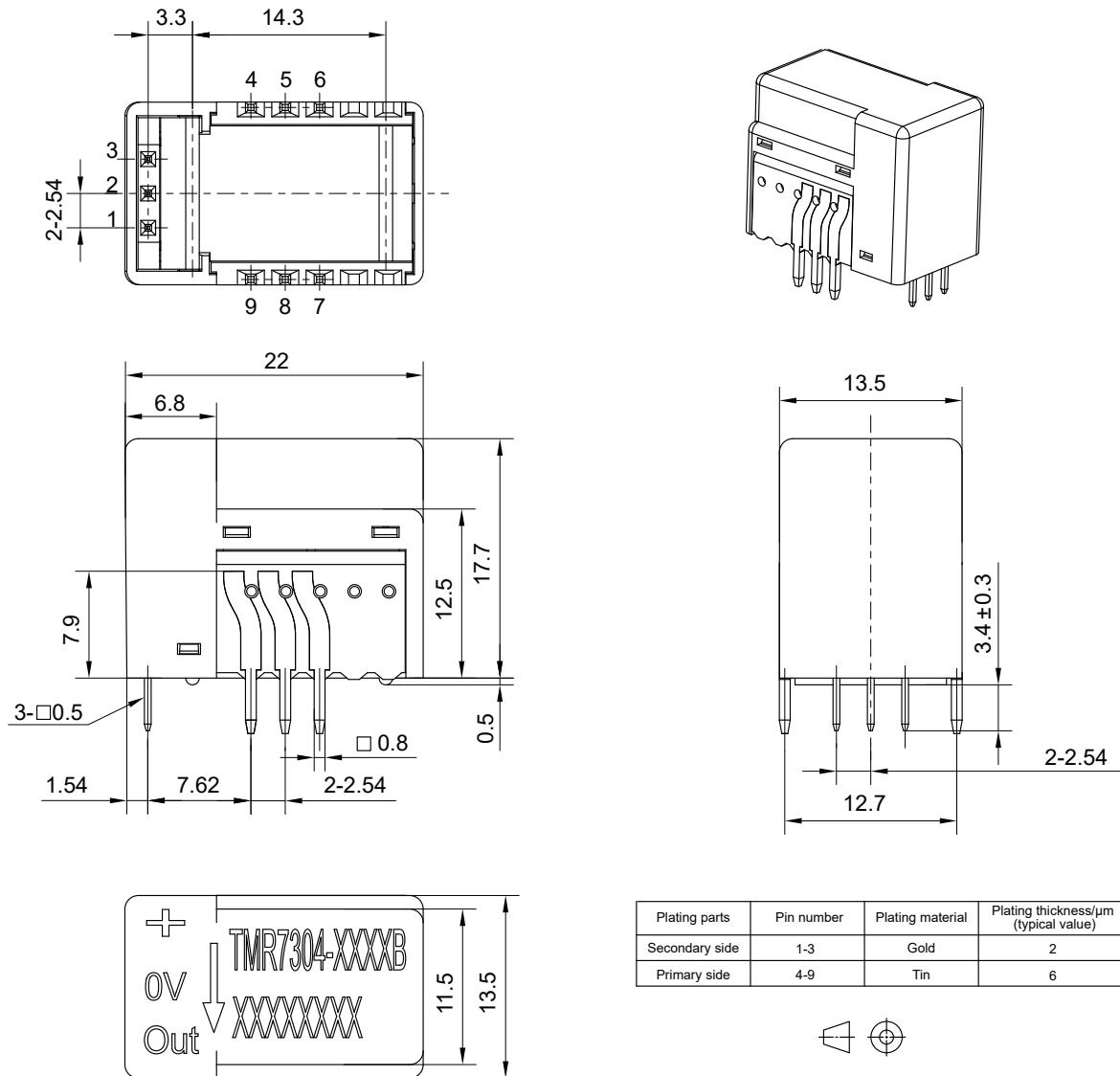
Figure 20. Dimension for TMR7304-B (unit: mm, tolerances for unmarked scales \pm 1 mm)
