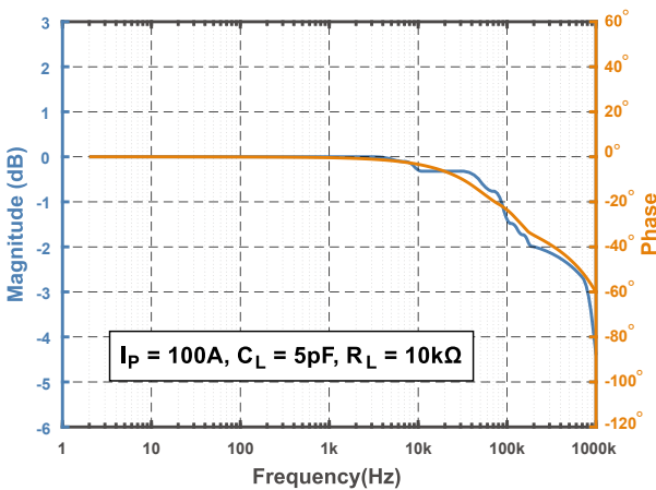
Figure 5. Bode Plot
