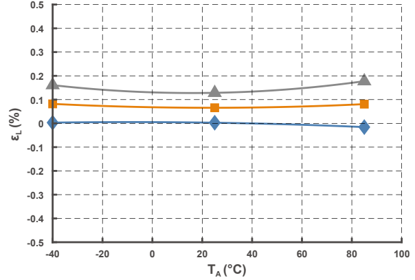
Figure 7. Linearity
