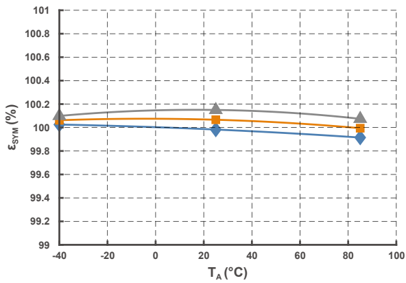
Figure 8. Symmetry
