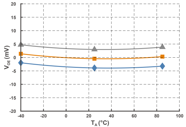
Figure 9. Offset Error
