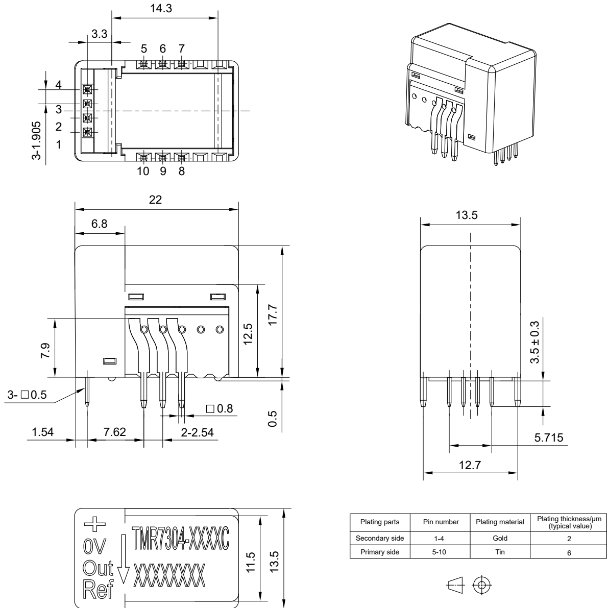
Figure 21. Dimension for TMR7304-C (unit: mm, tolerances for unmarked scales \pm 1 mm)
