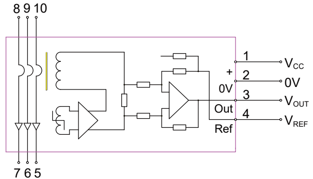
Figure 17. TMR7304-C Electrical Connection
