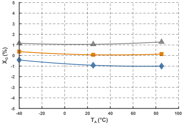
Figure 6. Accuracy
