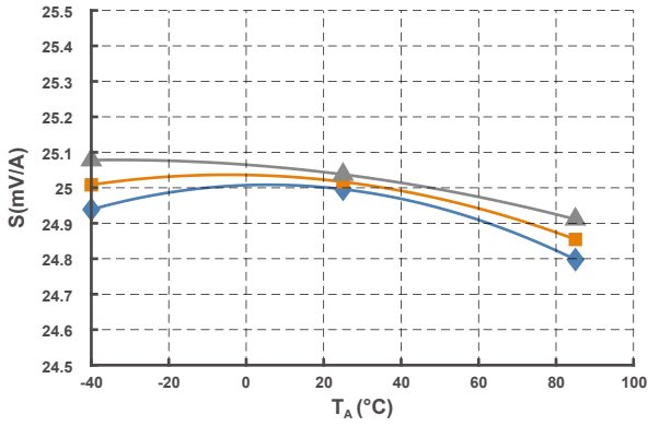
Figure 12. Sensitivity (@I PN = 25 A)
