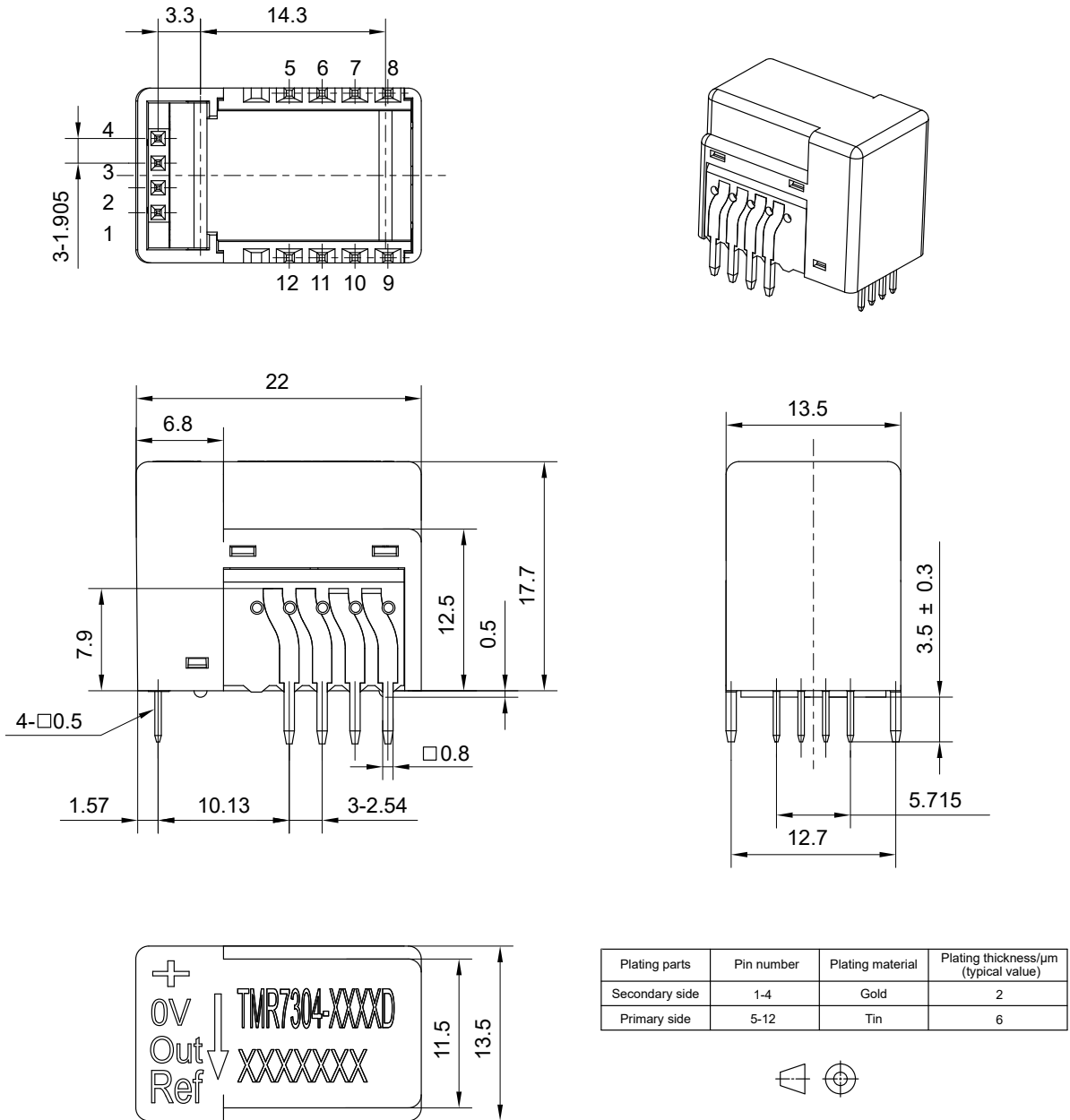
Figure 22. Dimension for TMR7304-D (unit: mm, tolerances for unmarked scales \pm 1 mm)
