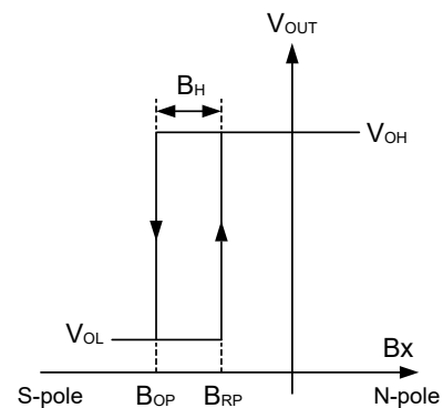
Figure 3. Switching characteristics
