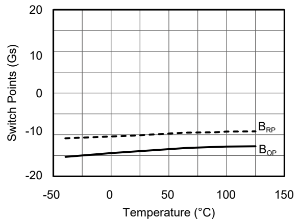
Figure 8. Switch points versus temperature ( V_{CC} = 3\text{ V} )
