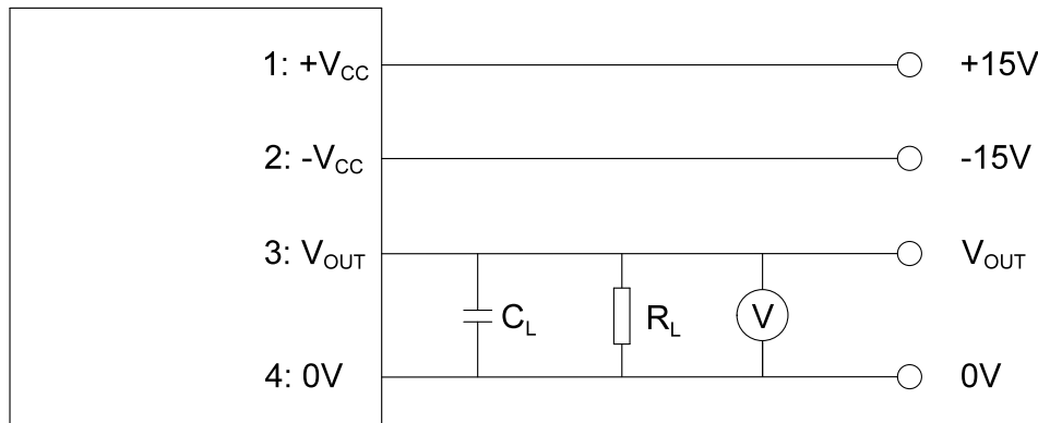
Figure 16. Connection diagram of TMR7503
