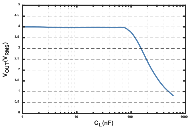
Figure 3. Output voltage versus load capacitance (@ I_P=I_{PN} )
