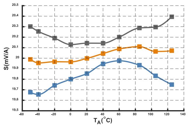
Figure 10. Sensitivity @ I_{PN} = 200 A versus ambient temperature
