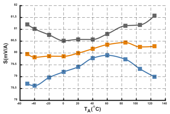
Figure 8. Sensitivity @ I_{PN} = 50 A versus ambient temperature
