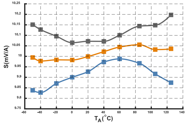
Figure 12. Sensitivity @ I_{PN} = 400 A versus ambient temperature
