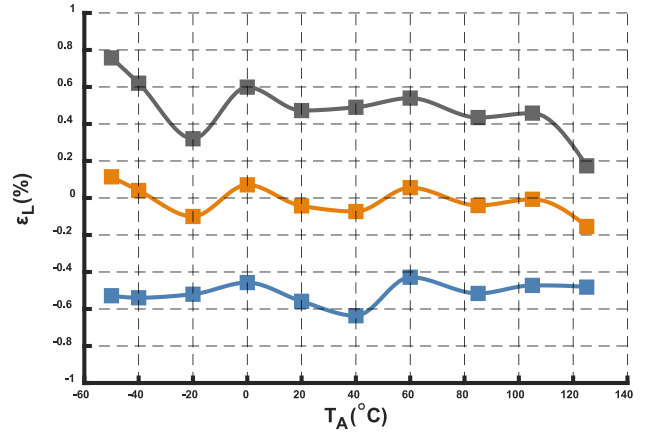
Figure 6. Linearity error versus ambient temperature
