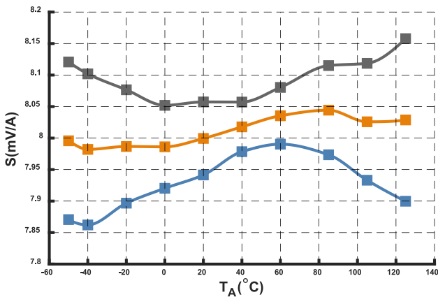
Figure 13. Sensitivity @ I_{PN} = 500 A versus ambient temperature
