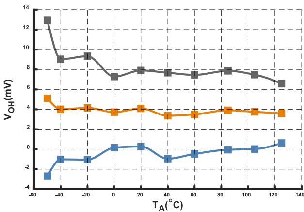
Figure 15. Hysteresis versus ambient temperature
