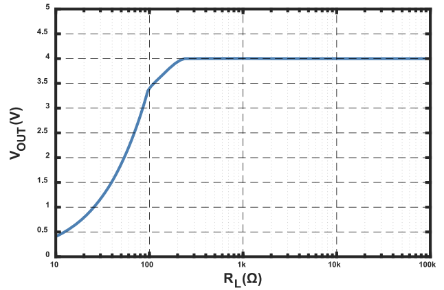
Figure 2. Output voltage versus load resistance (@ I_P=I_{PN} )
