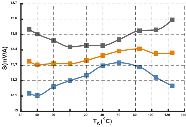
Figure 11. Sensitivity @ I_{PN} = 300 A versus ambient temperature
