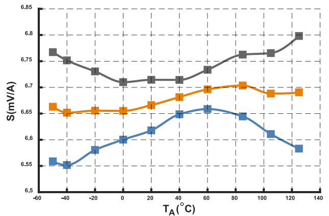
Figure 14. Sensitivity @ I_{PN} = 600 A versus ambient temperature
