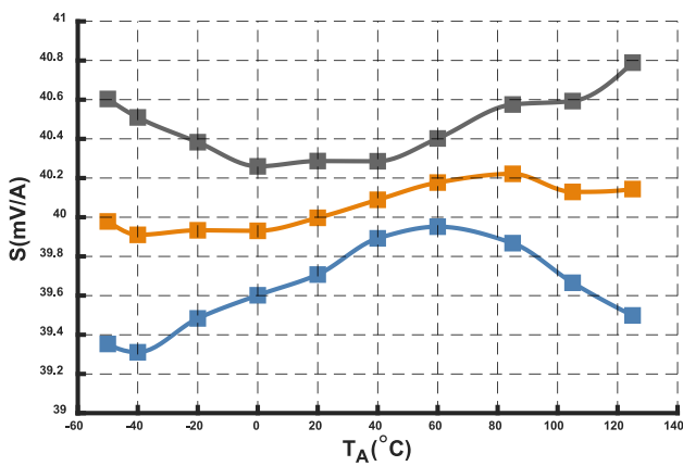
Figure 9. Sensitivity @ I_{PN} = 100 A versus ambient temperature
