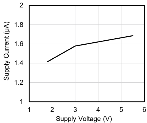
Figure 9. Supply current versus supply voltage (T A =25°C)
