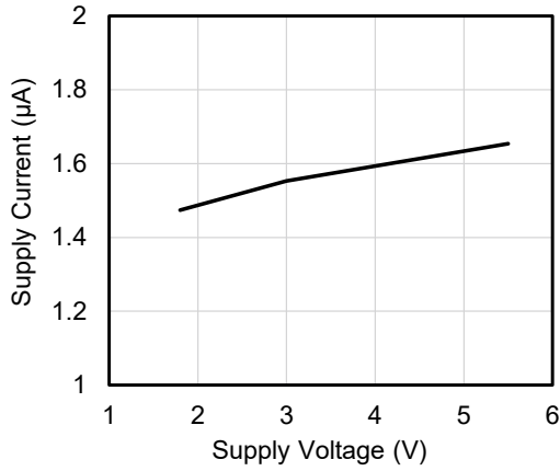
Figure 5. Supply current versus supply voltage (T A =25°C)
