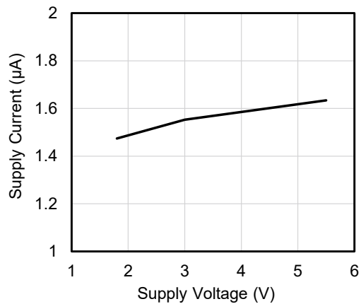
Figure 7. Supply current versus supply voltage (T A =25°C)
