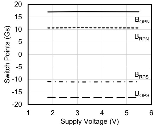
Figure 6. Switch points versus supply voltage (T A =25°C)
