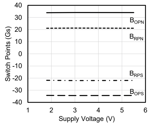
Figure 8. Switch points versus supply voltage (T A =25°C)
