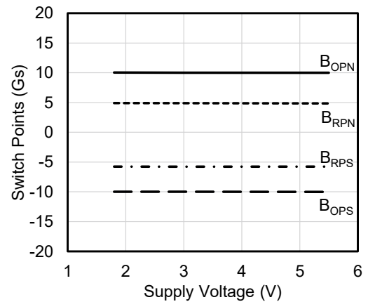
Figure 10. Switch points versus supply voltage (T A =25°C)
