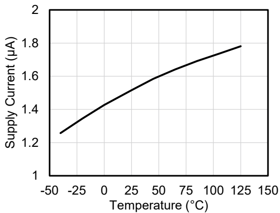
Figure 7. Supply current versus temperature (V CC = 3 V)
