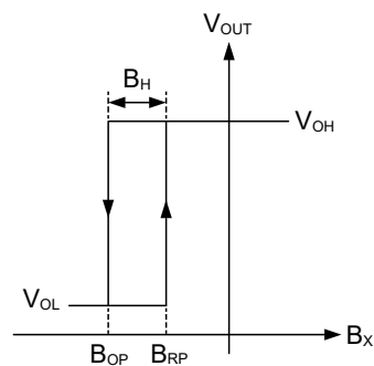
Figure 3. Switching characteristics
