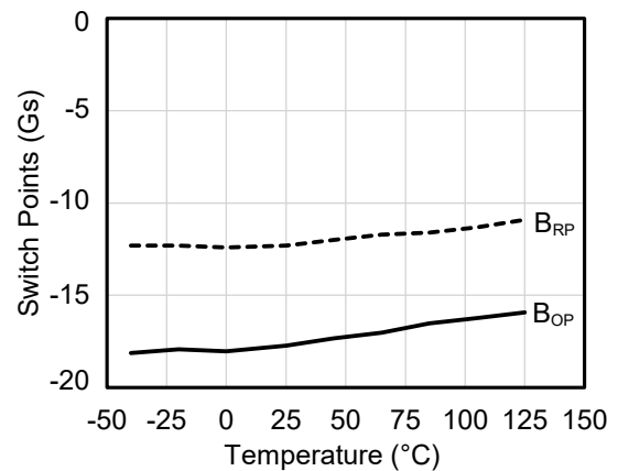
Figure 8. Switch points versus temperature (V CC = 3 V)
