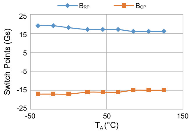
Figure 6. Switch points versus temperature ( V_{CC} = 3 \text{ V} )
