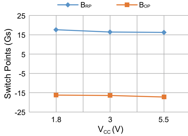
Figure 5. Switch points versus supply voltage ( T_A=25^\circ\text{C} )
