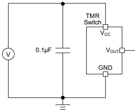
Figure 7. Application circuit diagram
