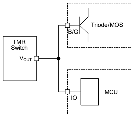
Figure 8. Application diagram for driving power load
