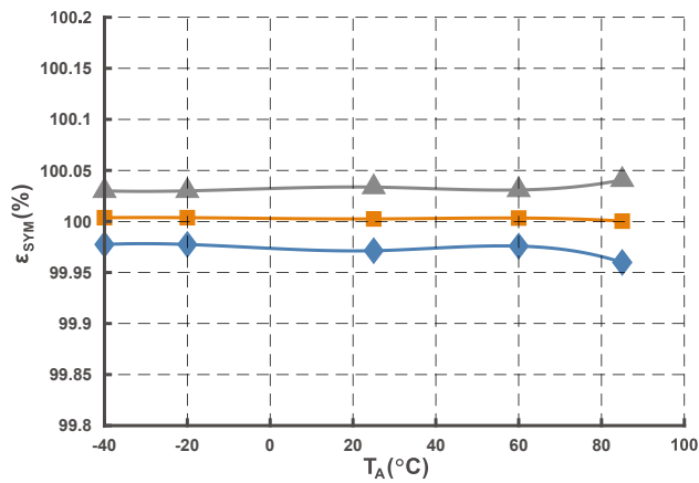
Figure 8. Symmetry
