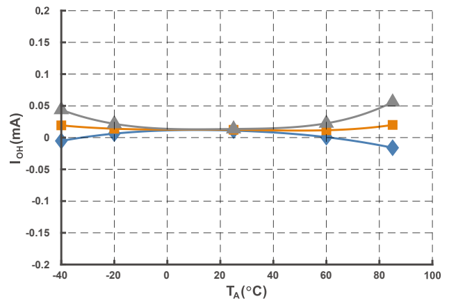
Figure 11. Hysteresis
