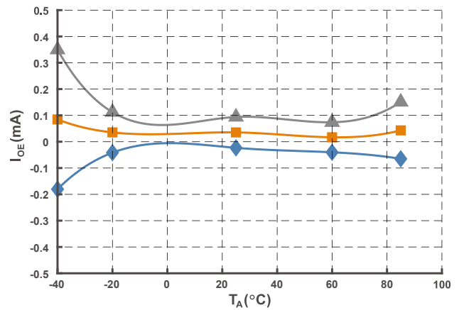
Figure 9. Offset Error
