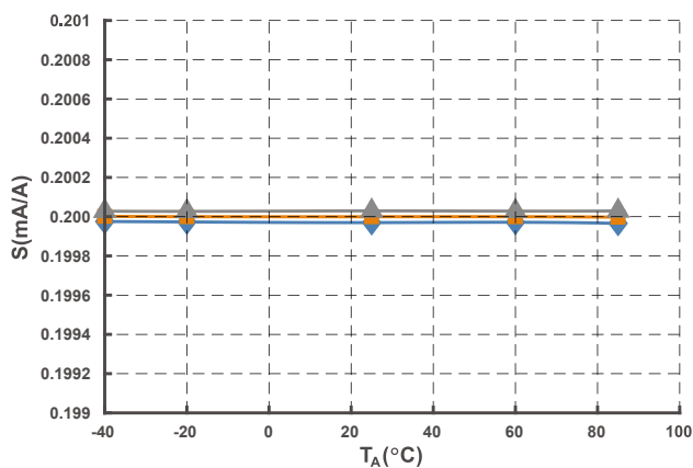
Figure 10. Sensitivity
