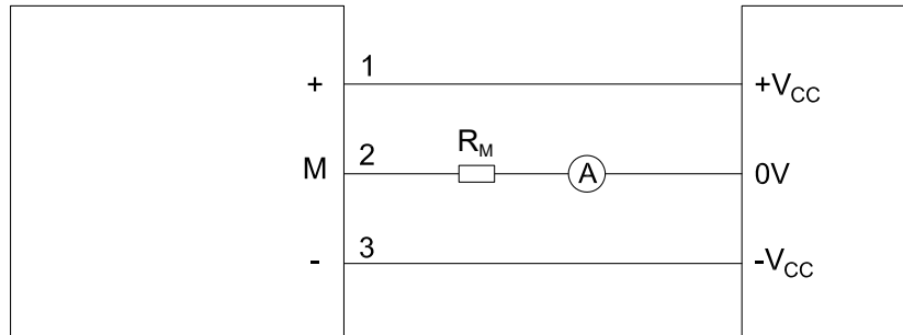
Figure 12. Electrical Connection
