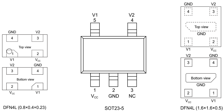
Figure 2. Pin configuration
