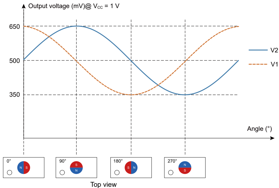
Figure 5-1. Single-ended output of TMR3015D in one period @ V_{CC} = 1\text{ V}
