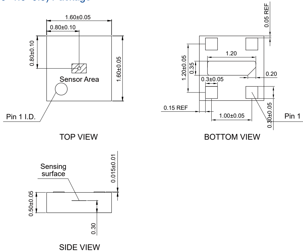
Figure 7. Package outline of DFN4L(1.6×1.6×0.5) (unit: mm)
