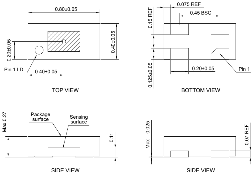
Figure 6. Package outline of DFN4L(0.8×0.4×0.23) (unit: mm)
