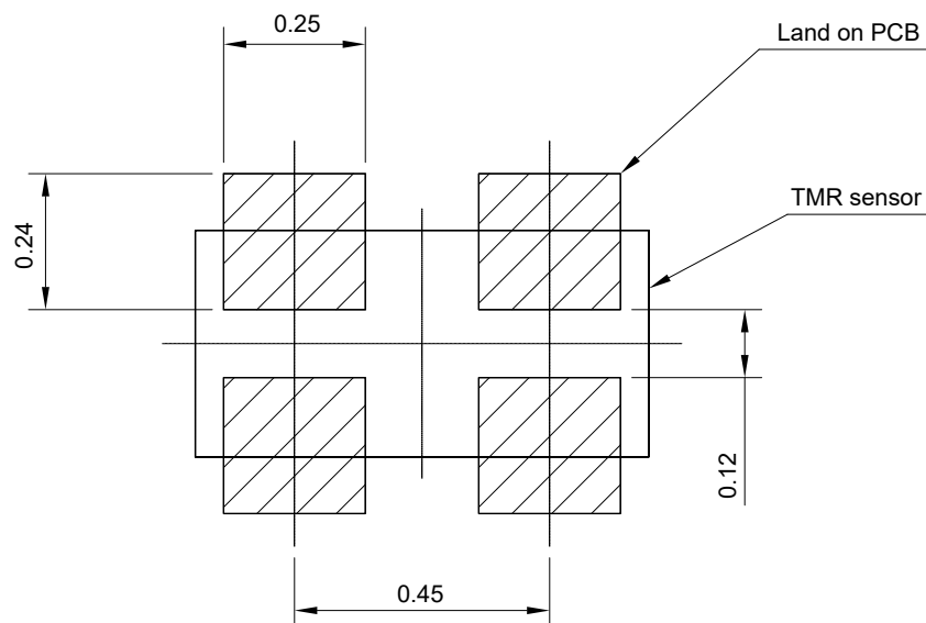
Figure 10. Recommended pad size diagram of DFN4L(0.8×0.4×0.23) (unit: mm)
