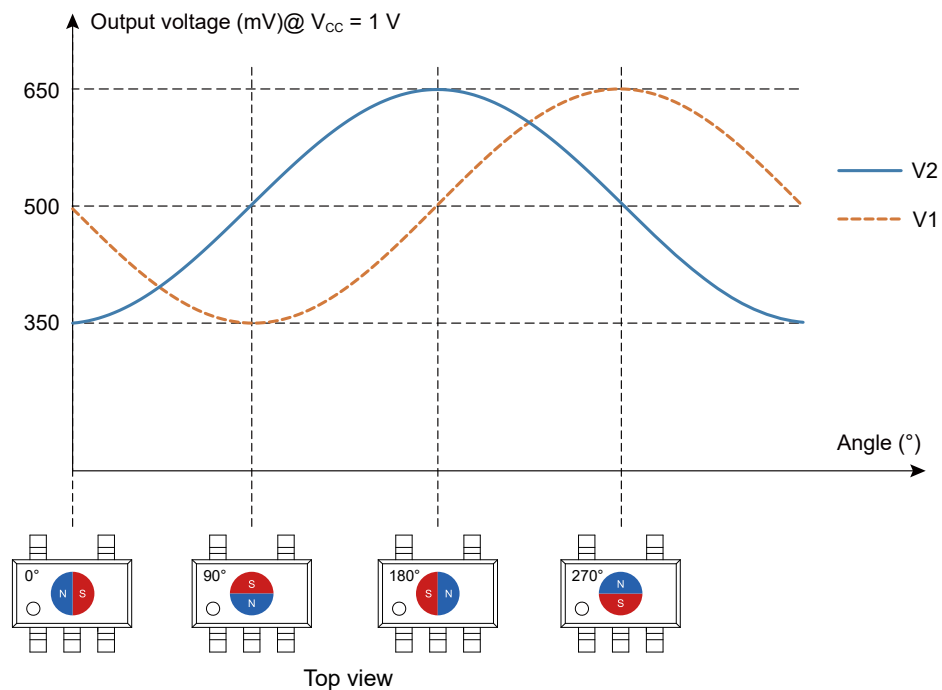
Figure 5-3. Single-ended output of TMR3015S in one period @ V_{CC} = 1\text{ V}
