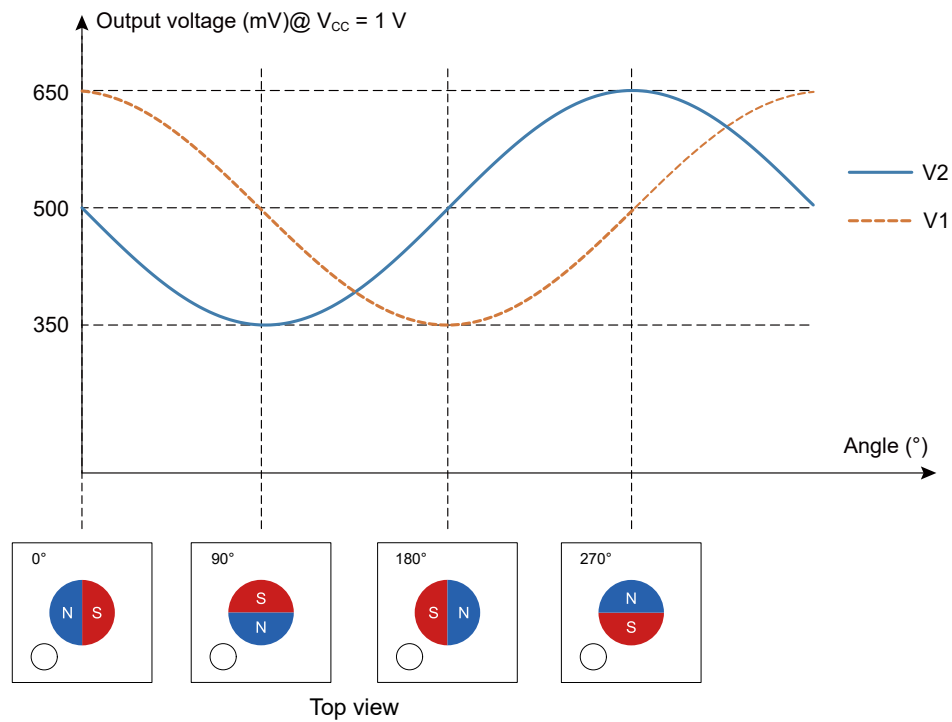
Figure 5-2. Single-ended output of TMR3015F in one period @ V_{CC} = 1\text{ V}
