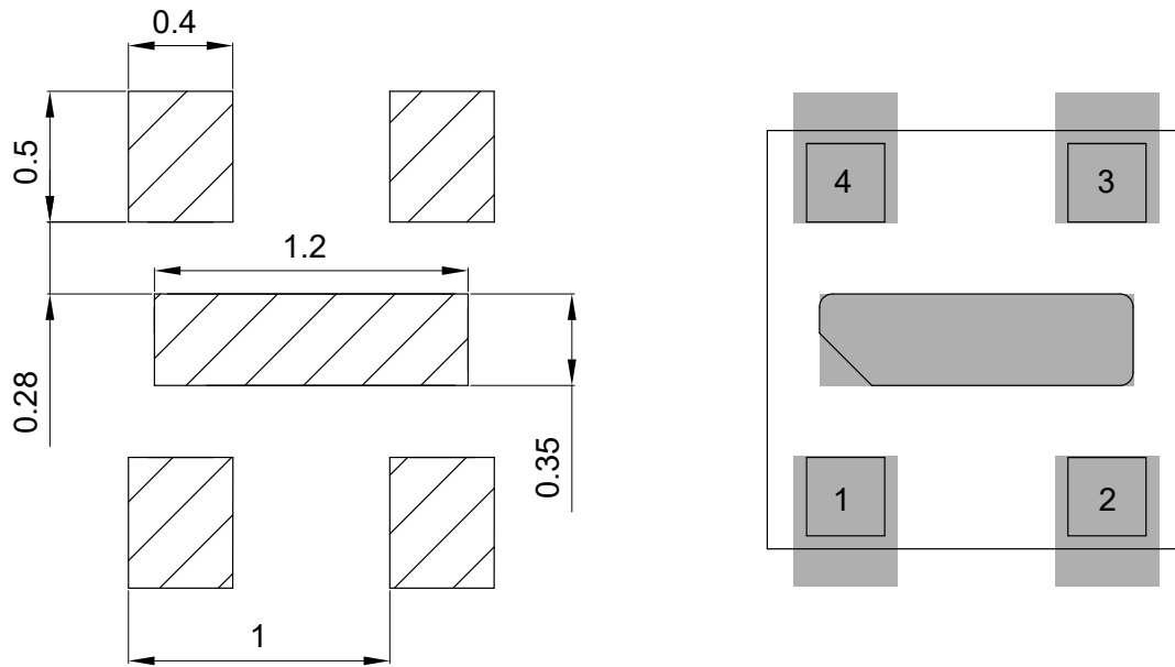
Figure 9. Recommended pad size diagram of DFN4L(1.6×1.6×0.5) (unit: mm)
