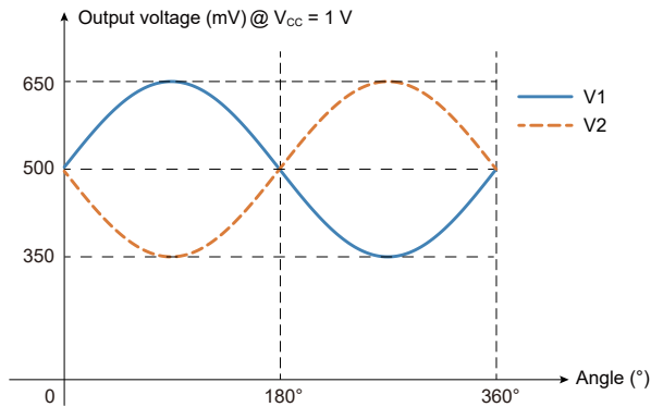
Figure 5. Single-ended output of TMR3014 in one period @ V_{CC} = 1\text{ V}
