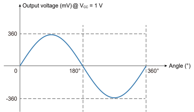
Figure 6. Differential output of TMR3014 in one period @ V_{CC} = 1\text{ V}
