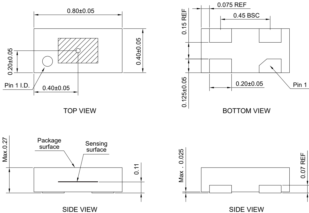
Figure 7. Package outline of DFN4L (unit: mm)
