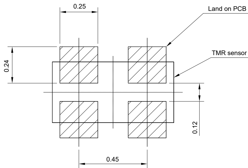
Figure 8. Land Pattern (Reference) (unit: mm)
