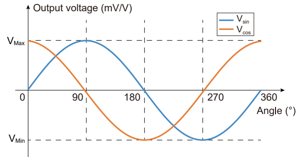
Figure 5. Output curve
