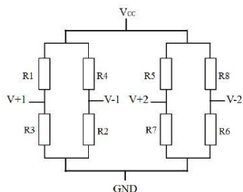
Dual-Bridge Configuration
