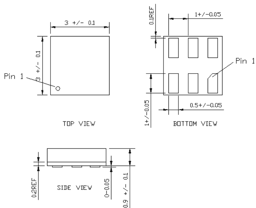
LGA6L (3x3) package drawing:
