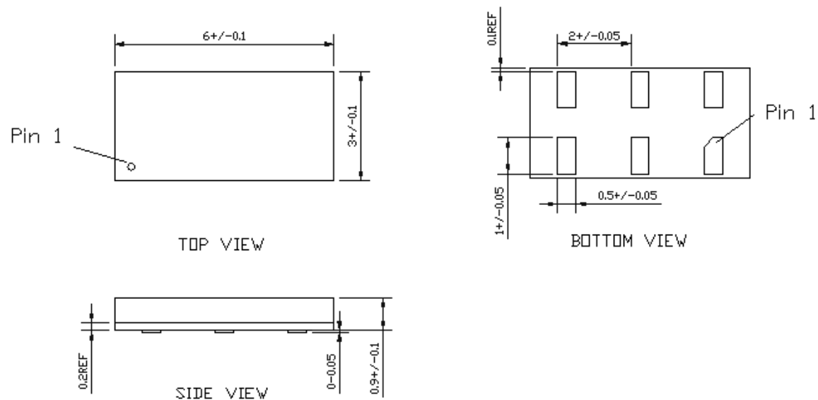
LGA6L (3x6) package drawing:
