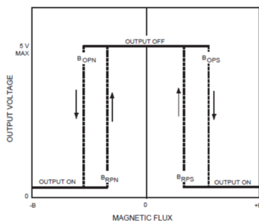
Magnetic Flux
